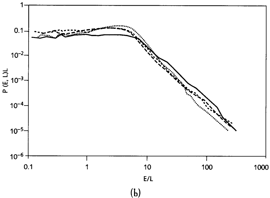
Figure 17. (a) Distribution of the size E of avalanches in rice piles of different lengths L . The various curves are for various sizes of rice piles. By systematically shifting the curves, they can be brought to cover each other (b). This property is known as finite size scaling, and implies criticality (Frette et al., 1995).
